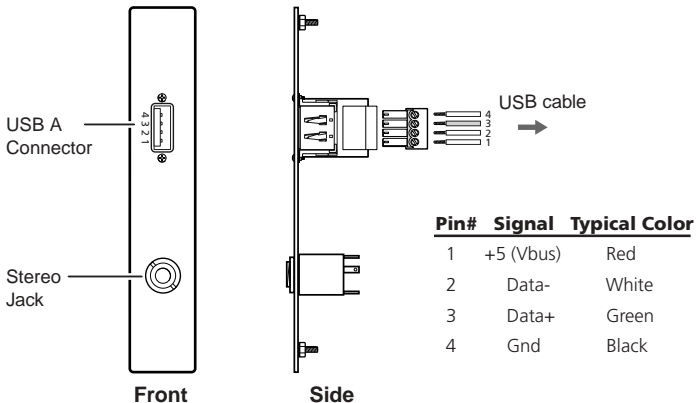
USB A to Captive Screw AAP/MAAP
