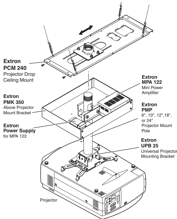
Figure 2 — A typical projector mounting installation, using an Extron PCM 240, a PMK 350, a PMP, and a UPB 25 Universal Projector Mounting Bracket
