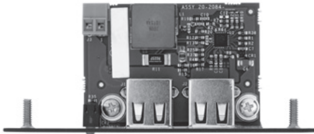
Top View - USB PowerPlate 200 AAP
